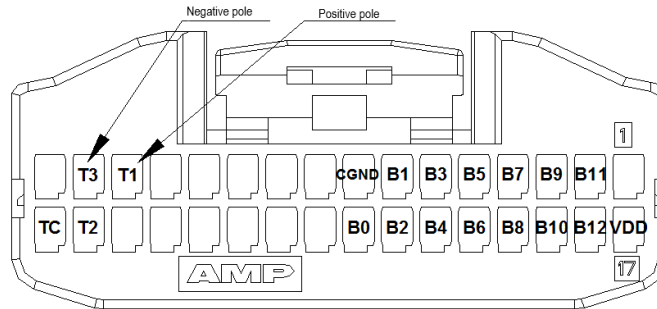
B12/VDD/T1--Battery positive pole B0/CGND/T3--Battery negative pole
